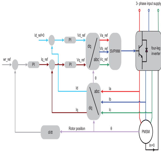
Fig 2 Control structure of four-leg PMSM drive under healthy operating condition
