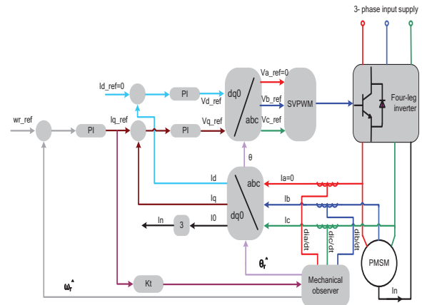
Fig10. the sensorless vector control structure for the four-phase inverter PMSM drive under a phase 'b' open-circuit fault.
