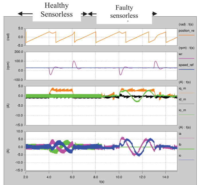
Fig 13 Fully Sensorless half load Steps under healthy condition and under open phase a fault condition.
