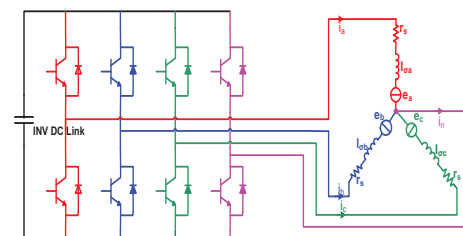
Fig1 The fault tolerant two level four-leg converter motor drive configuration.
