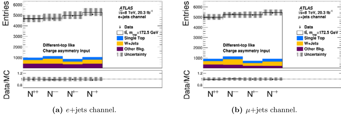
Figure 4. Different-top-like charge-pairings distributions. The hashed area represents all experimental systematic uncertainties as well as the b -hadron production and hadron-to-muon branching ratio uncertainties. The lower panel of the distributions show the ratio of the data divided by the simulation. (a) shows the e+jets channel while (b) shows the \mu+jets channel.
