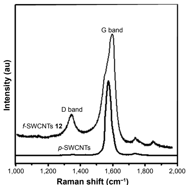
Figure 2 Raman spectra of p -SWCNTs and f -SWCNTs 12 . Abbreviations: f -SWCNTs, functionalized single-walled carbon nanotubes; p -SWCNTs, pristine single-walled carbon nanotubes.
