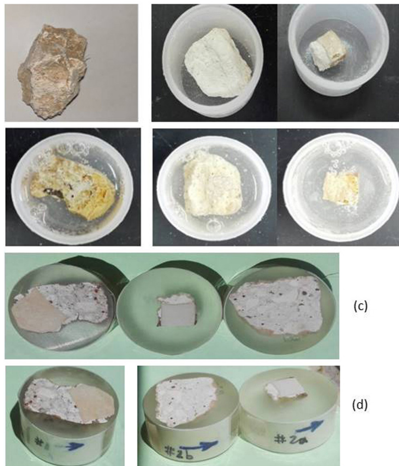
FIG. 11. Samples preparation for microscopic examination: a) Samples 1, 2a and 2b cut and placed in cups; b) epoxy is poured on samples for consolidation and grinding; c) samples ground and polished; (d) orientation of samples with respect to mosaic surface taken, arrows point to upper surface.
