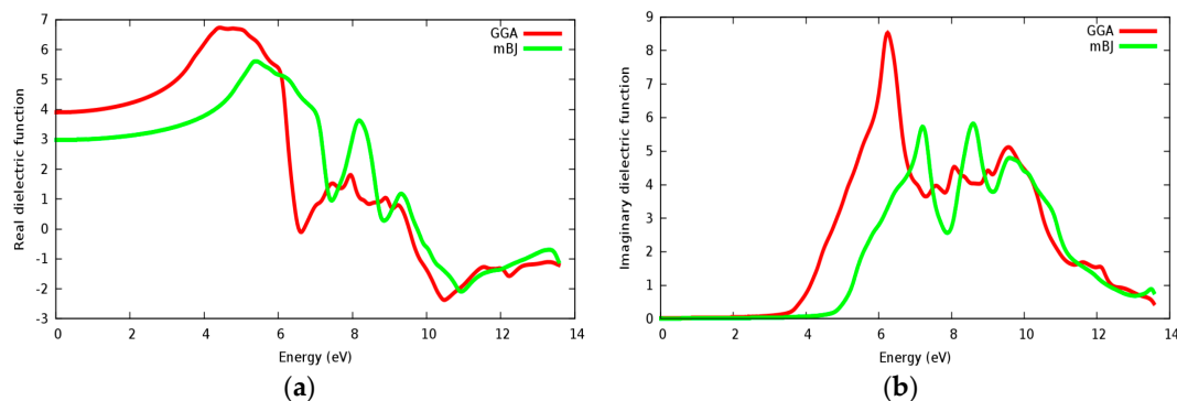
Figure 14. Dielectric function for SrZrO 3 : (a) Real part; (b) Imaginary part using both PBE-GGA and mBJ-GGA methods.
