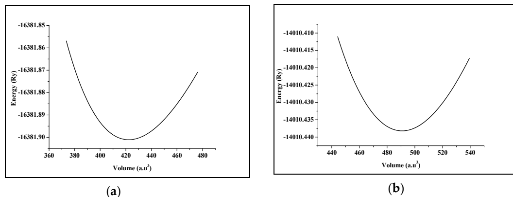
Figure 2. Total energy as a function of the volume of (a) \text{SrRhO}_3 compound and (b) \text{SrZrO}_3 compound.
