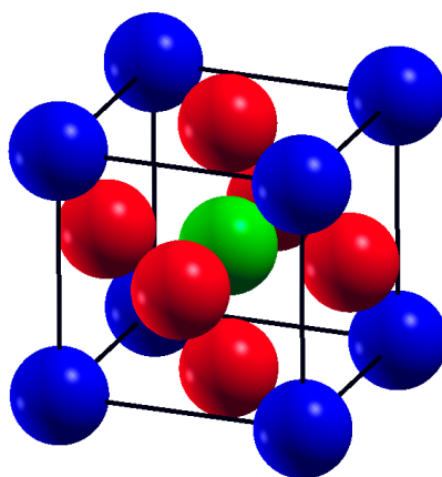
Figure 1. The crystal structure of \text{SrTMO}_3 (TM = Rh, Zr), (blue spheres are Sr atoms, red spheres are Oxygen O atoms and green spheres are TM atoms).
