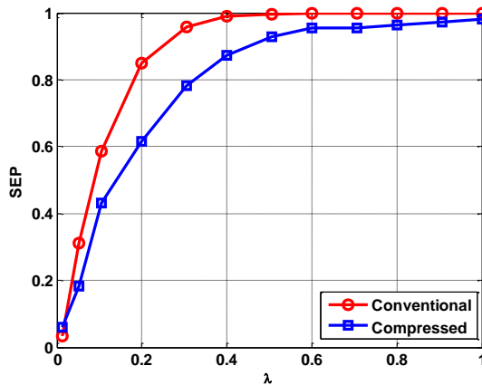
Fig. 11. Performance comparison: 16PPM modulation schemes using different values of \lambda
