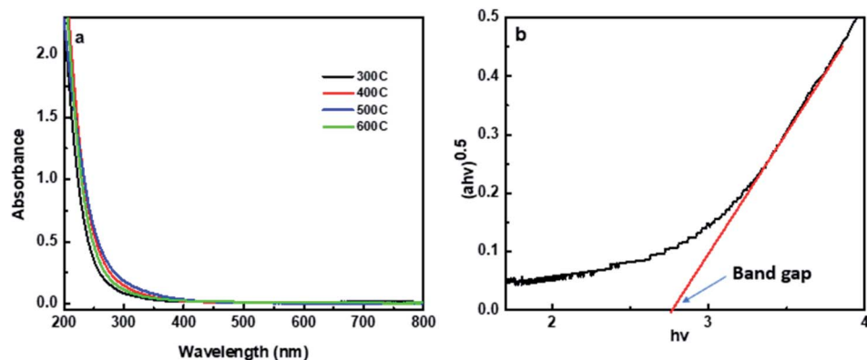
Fig. 6 (a) The absorption spectra of the prepared CNDs, and (b) Tauc plot of CD300.
