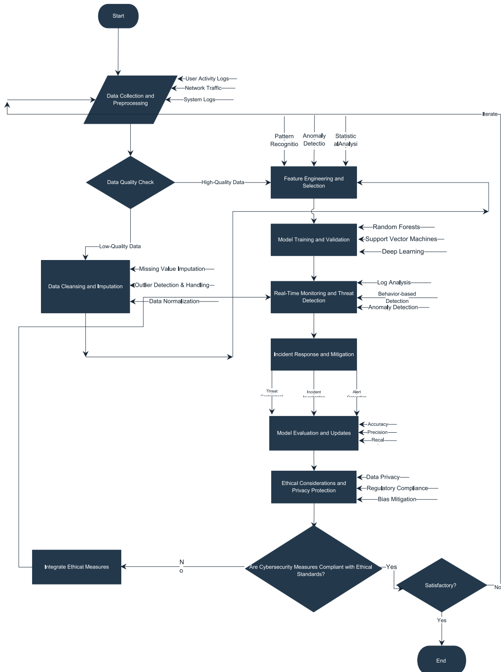
Fig. 2. Machine learning and cybersecurity integration model.
