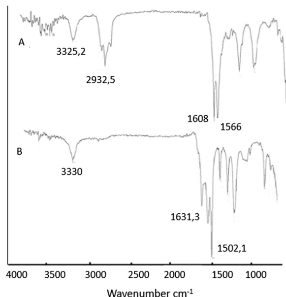
Fig. 4 FT-IR spectra of a LHM-DIC and b LPD-C after Pb(II) binding
