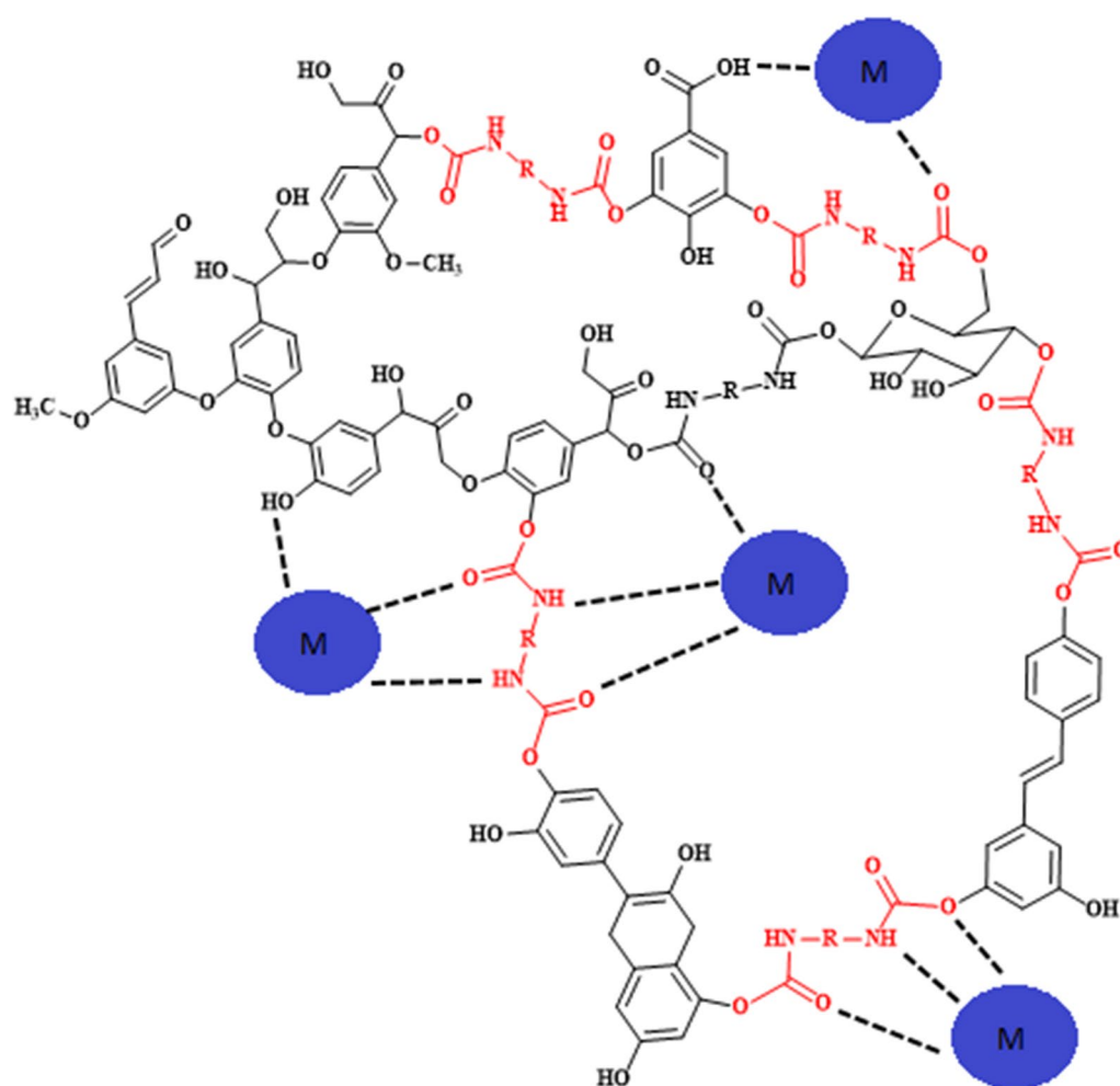
Scheme 1 A schematic diagram showing the binding sites in LHMDIC and LPDIC
