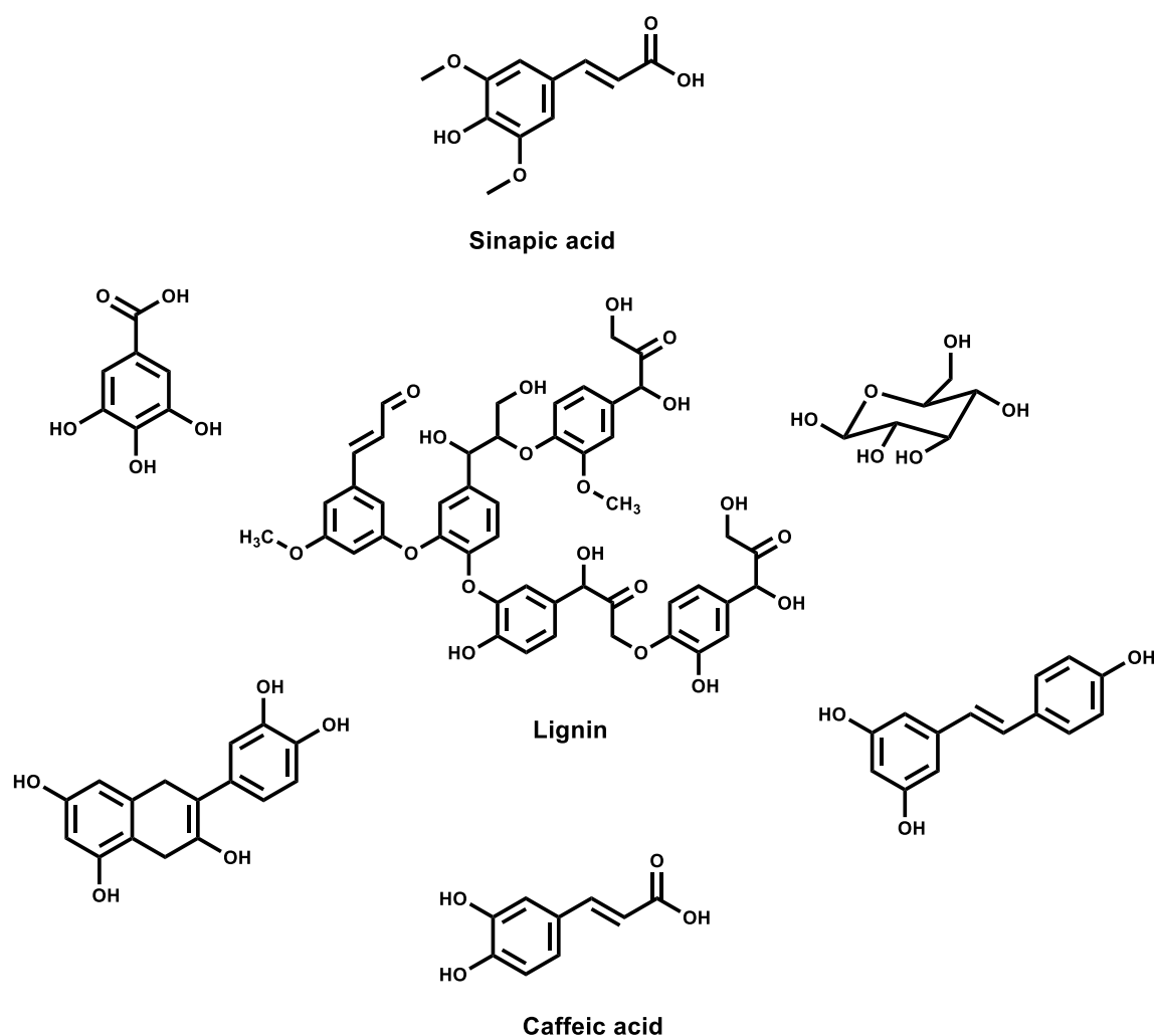
Fig. 1 Chemical structures OILW components
