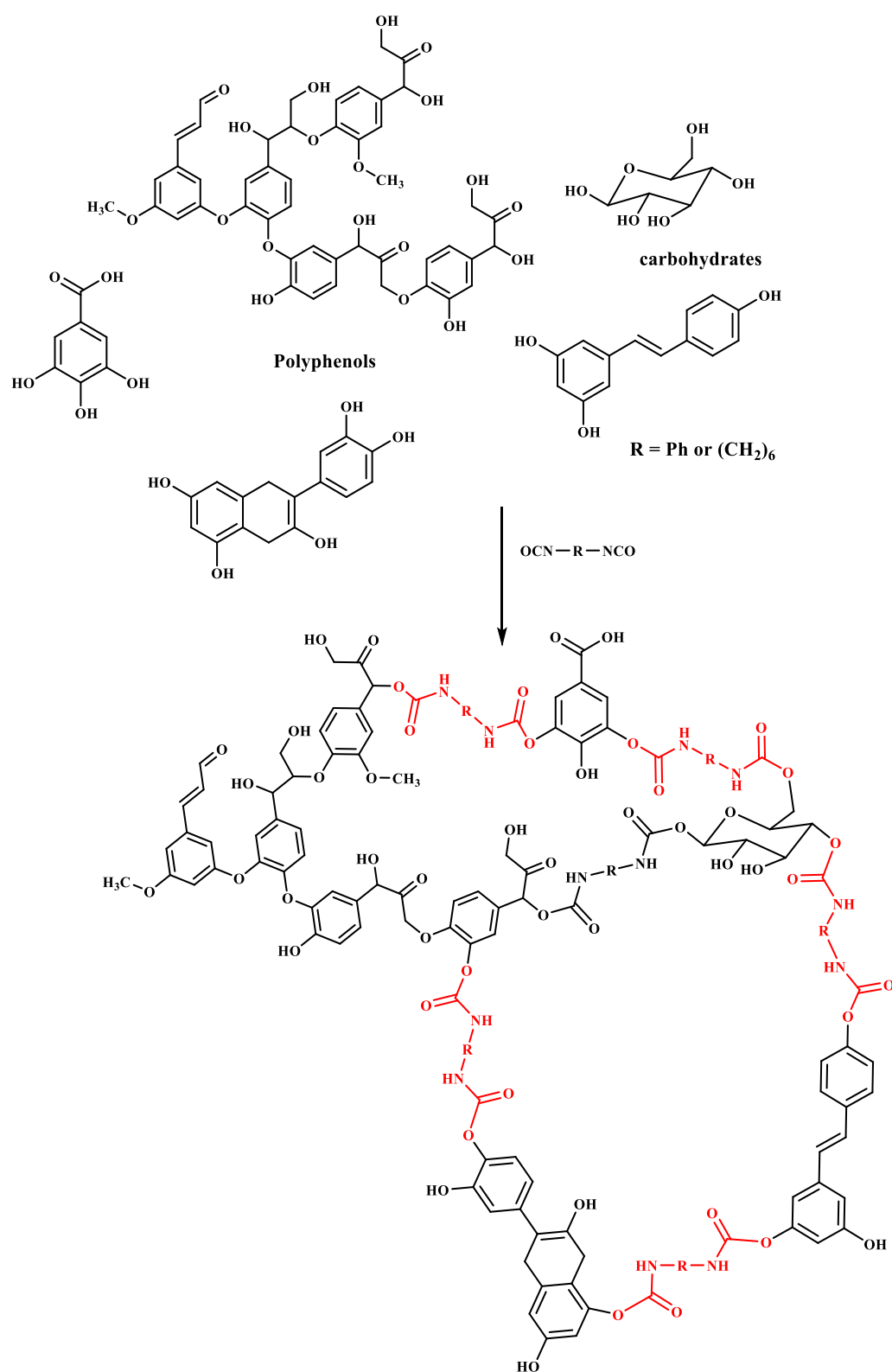
Fig. 2 A representative chemical structure of foam generated from polymerizing OILW and diisocyanates
