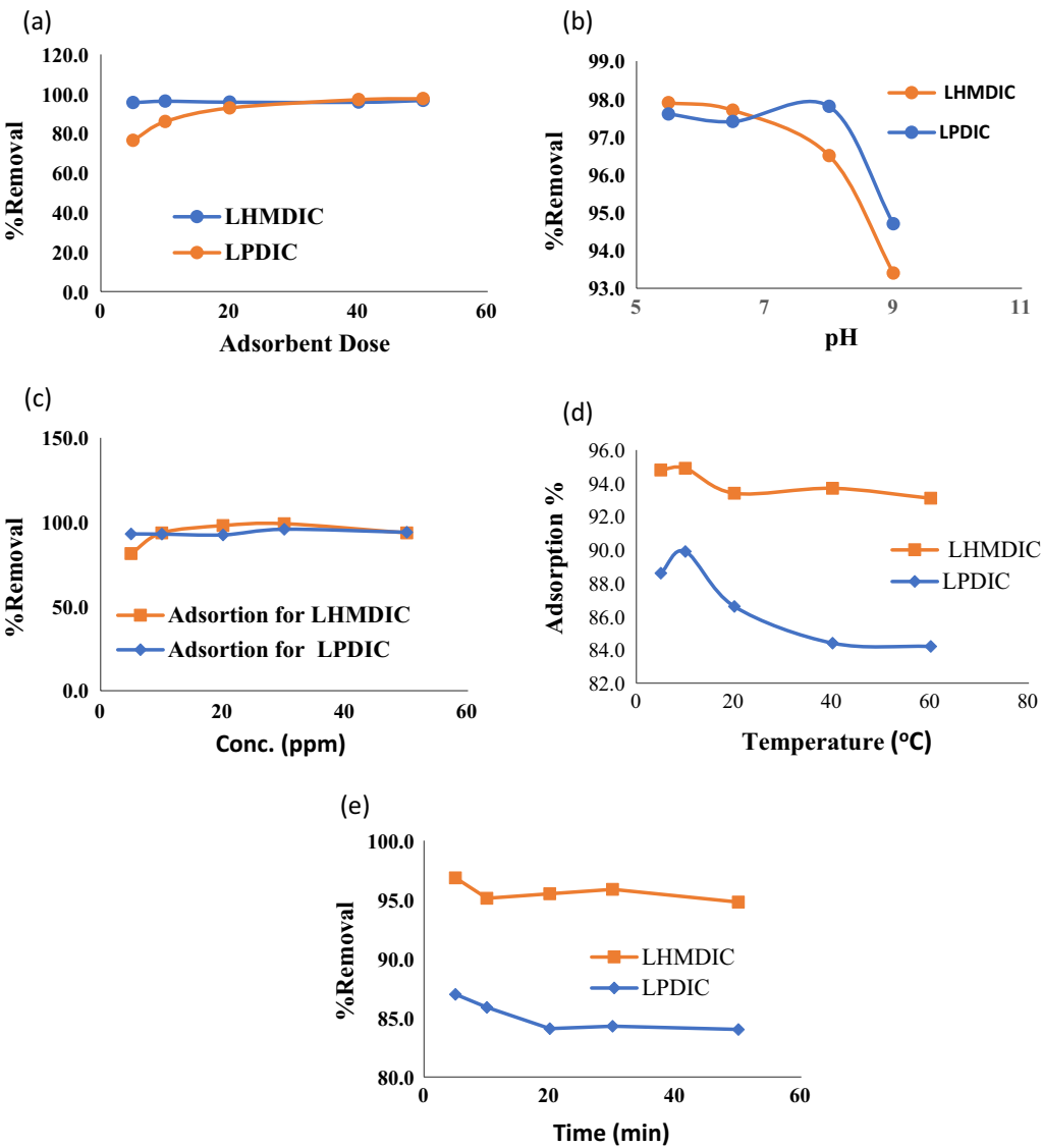
Fig. 7 The effect of a Foam dose b pH value c metal starting concentration d Temperature e mixing time
