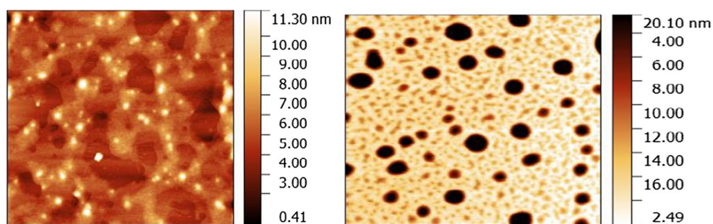
Fig. 5 AFM image of LHMDIC and LPDIC, respectively
