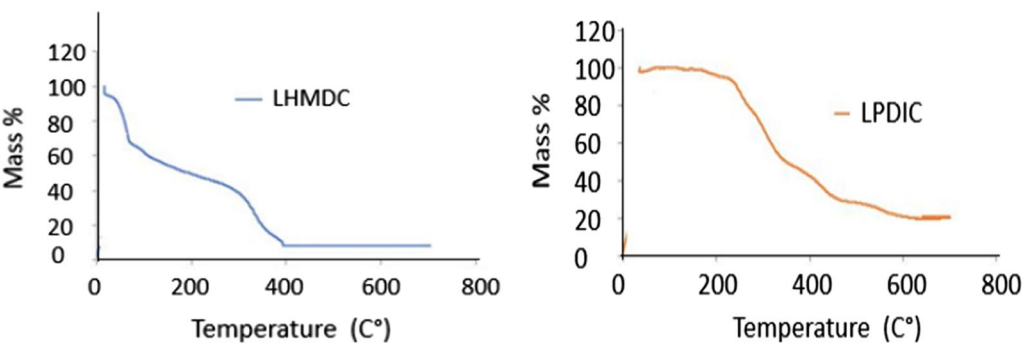
Fig. 6 Thermal gravimetric analysis of LHMDIC and LPDIC
