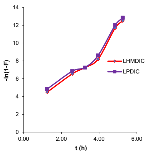
Fig. 11 Liquid film diffusion model plot for the Pb(II) adsorption by LHMDIC and LPDIC foams
