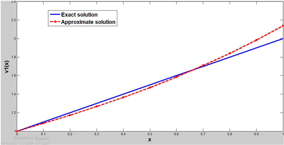
Figure 1. The exact and approximate solutions of v_1(x) using Algorithm (5.3) for system (5.1) with m = 3 .
