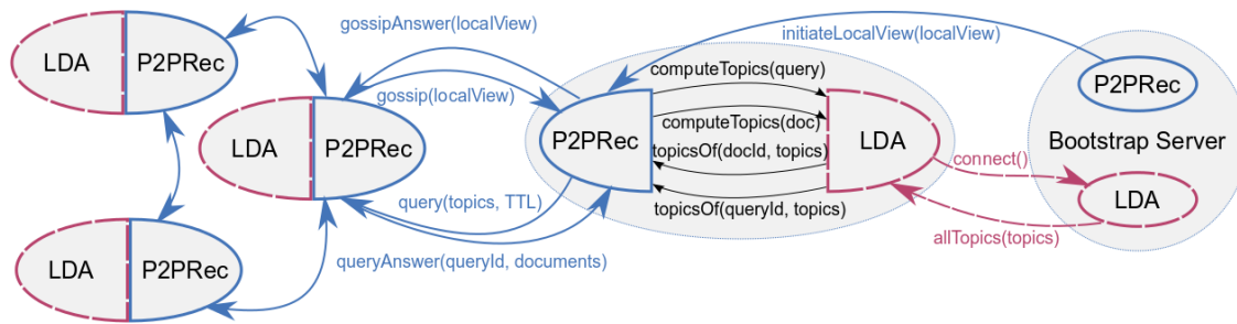
Figure 1: P2Prec Architecture.
